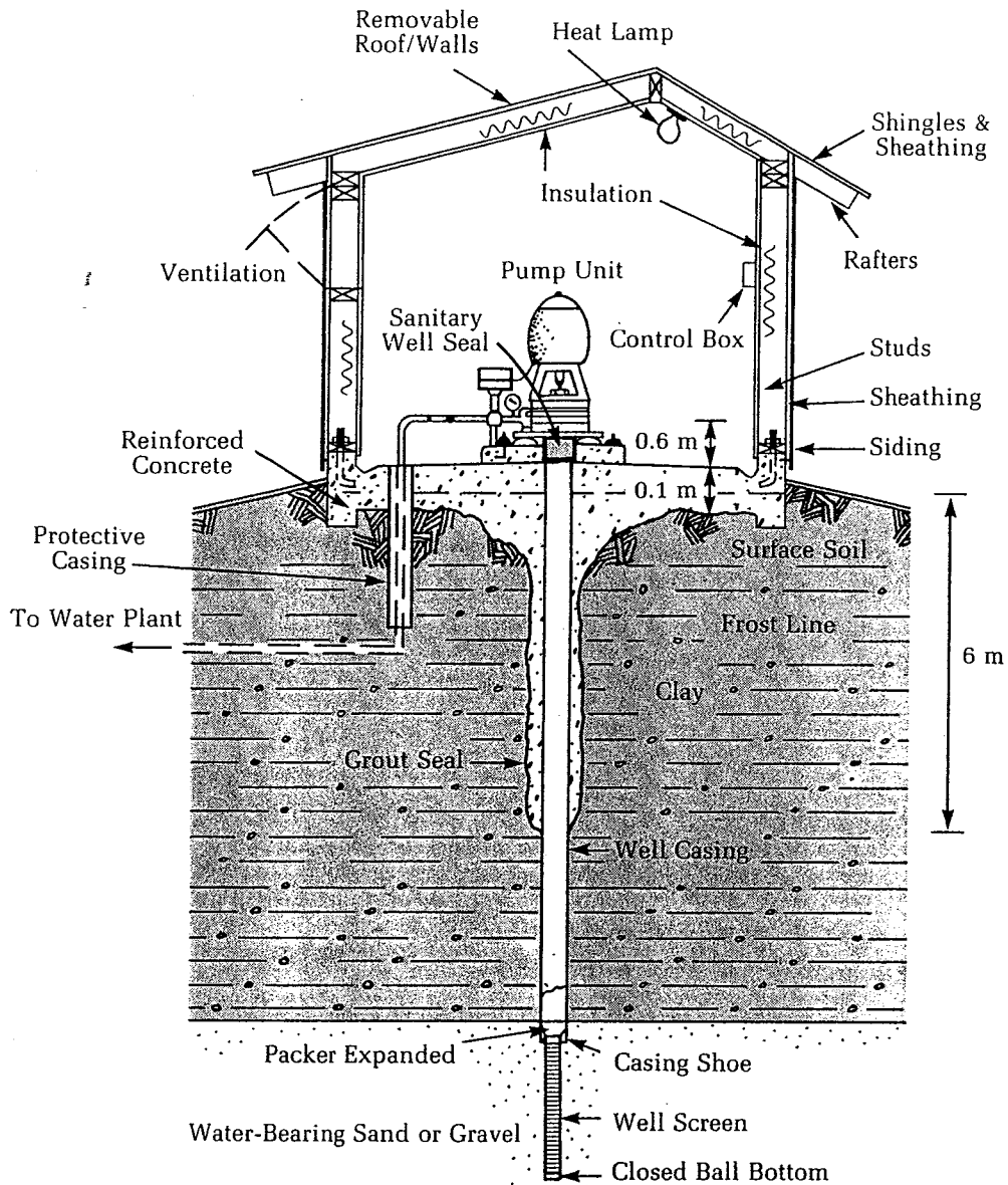
Figure 2-33 Pumphouse (Source: U.S. Environmental Protection Agency, Manual of Individual Water Supply Systems . See sourcenote for Figure 2-22 for publication data.)
