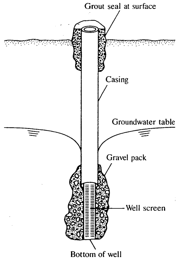
Figure 3-8 Typical well installation in an unconfined aquifer
