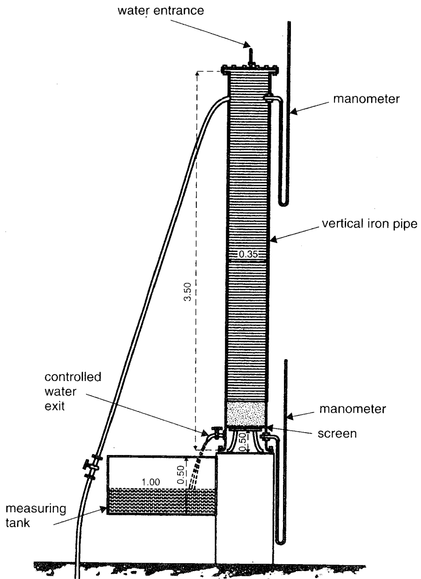
FIGURE 2.14. Apparatus intended to determine the law of the water flow through sand.
