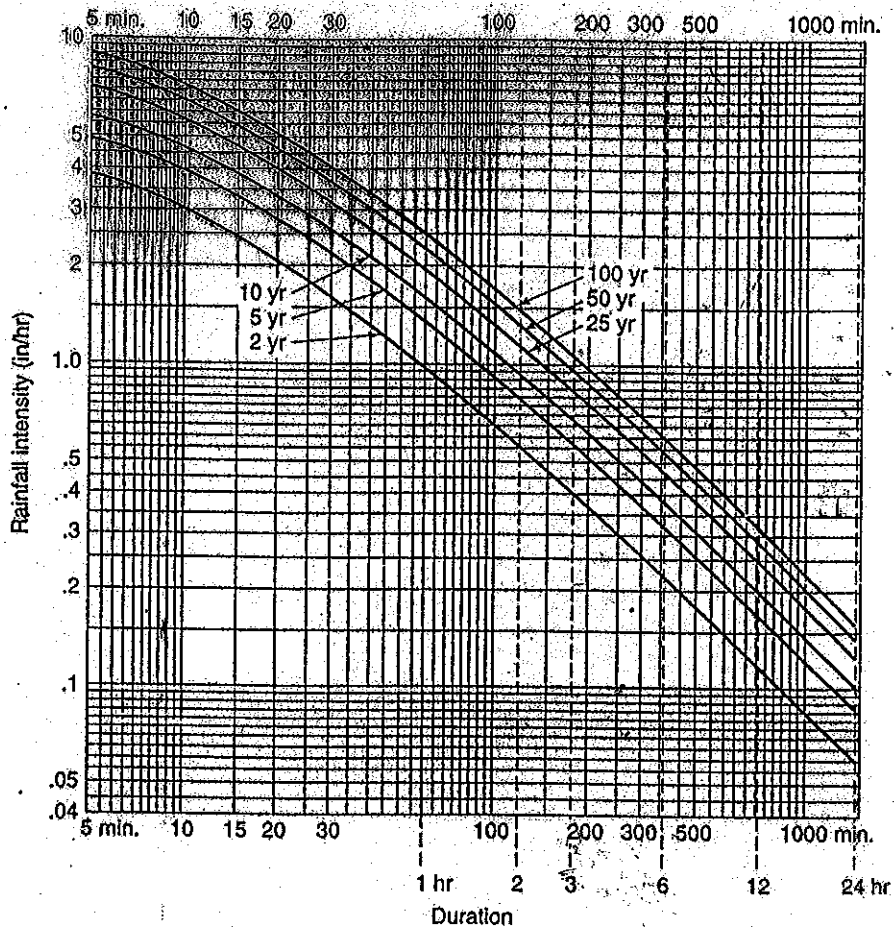
Figure 7.2.15 Rainfall intensity-duration-frequency relation (Phoenix metro area) (from Flood Control District of Maricopa County (1992)).
