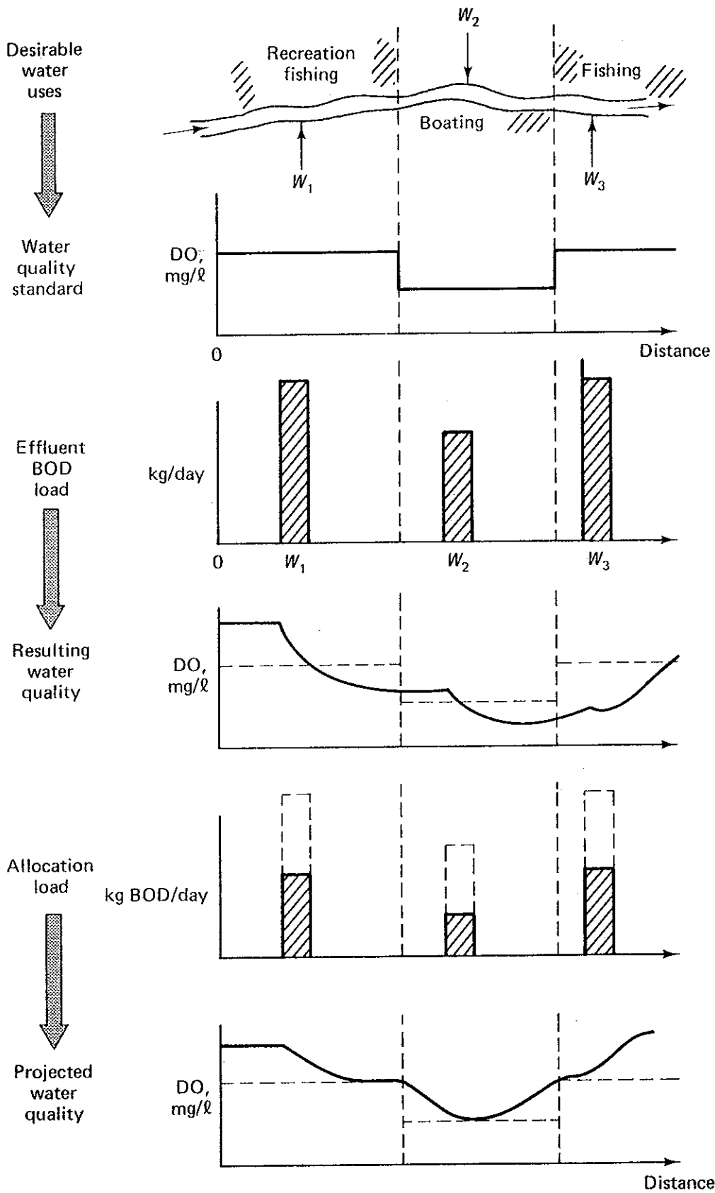
Figure 1.2 Representation of waste load allocation problem for dissolved oxygen.
