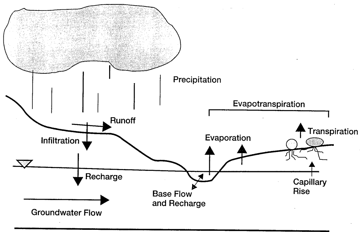
FIGURE 1.4.1 Schematic view of the hydrologic cycle
