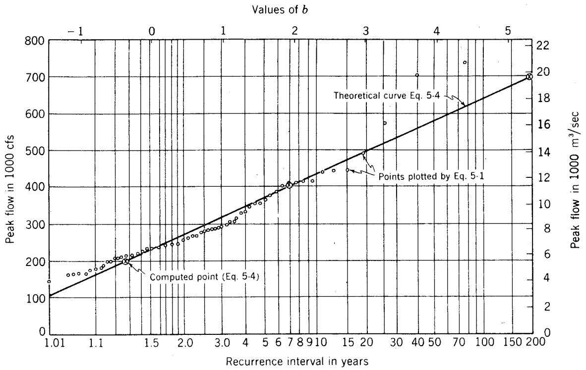
FIGURE 5.3 Frequency curve of annual floods for the Susquehanna River at Harrisburg, Pennsylvania (1874–1949).
