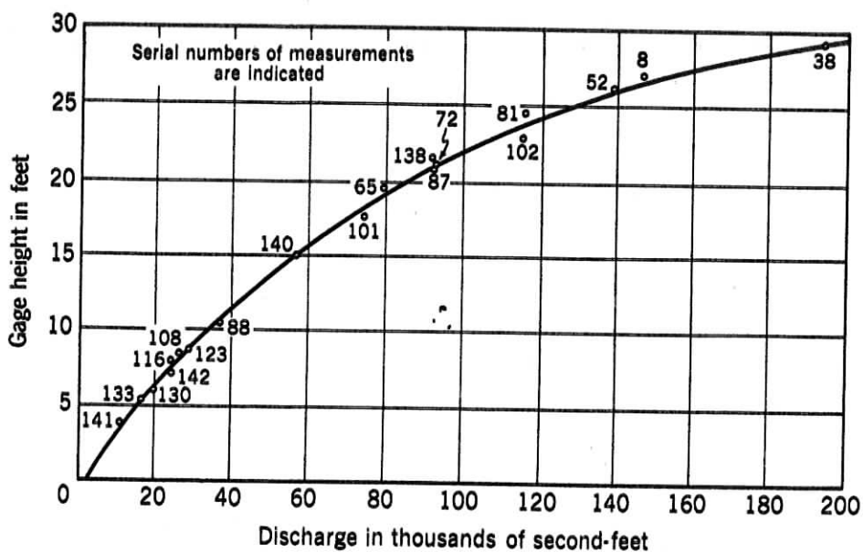
Figure 2-8 Stage-discharge relation for the Willamette River at Albany, Oregon. (Data from the U.S. Geological Survey)
