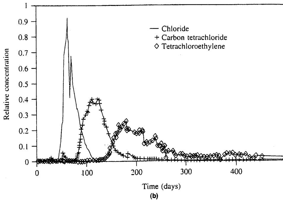
Figure 7.3 (a) Predicted advance of solutes in a one dimensional transport evaluation. (b) Observed field retardation data from the Borden landfill site, 5 meters downgradient from the injection well. Chloride is a non-sorbing tracer. Carbon tetrachloride and tetrachloroethylene are retarded by sorption.
