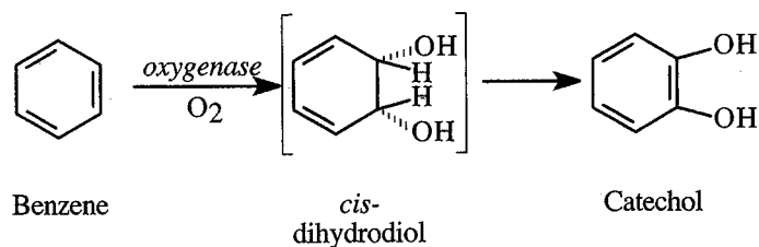
Figure 7.7 Enzymatic oxidation of benzene to catechol. The first step of benzene metabolism under aerobic conditions.
