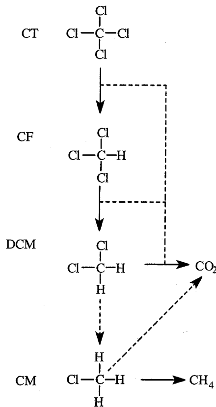
Figure 7.8 Pathway for the anaerobic metabolism of chlorinated methanes. Initial metabolism of carbon tetrachloride (CT) and chloroform (CF) metabolism are reduction to the level of dichloromethane (DCM). Subsequent metabolism results eventually in \text{CO}_2 production, although traces of chloromethane (CM) may accumulate as an intermediate. Source: Egli, et al., 1988; Freedman and Gossett, 1991; Galli and McCarty, 1989.
