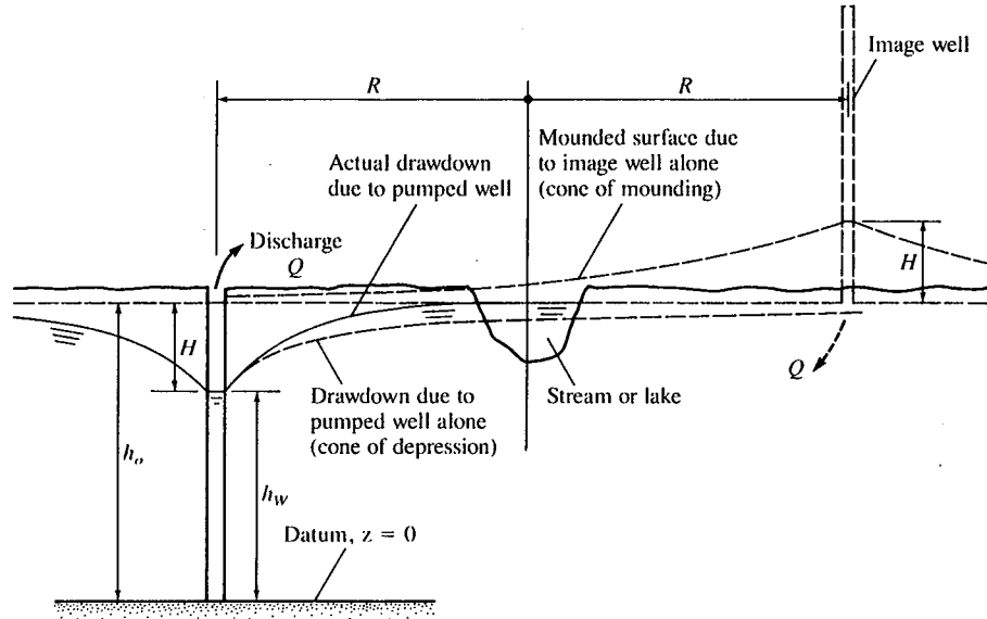
Figure 3-13 Analysis of drawdown for a pumped well near a recharging body of water
