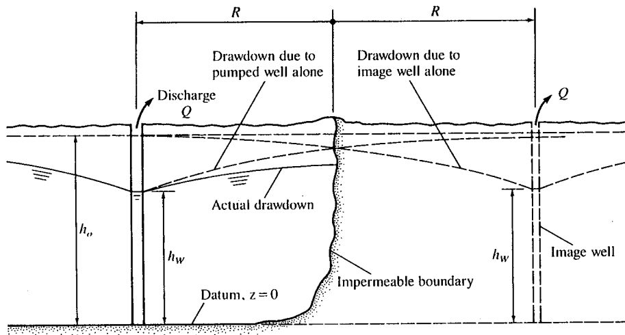
Figure 3-14 Analysis of drawdown for a pumped well near an impermeable barrier
