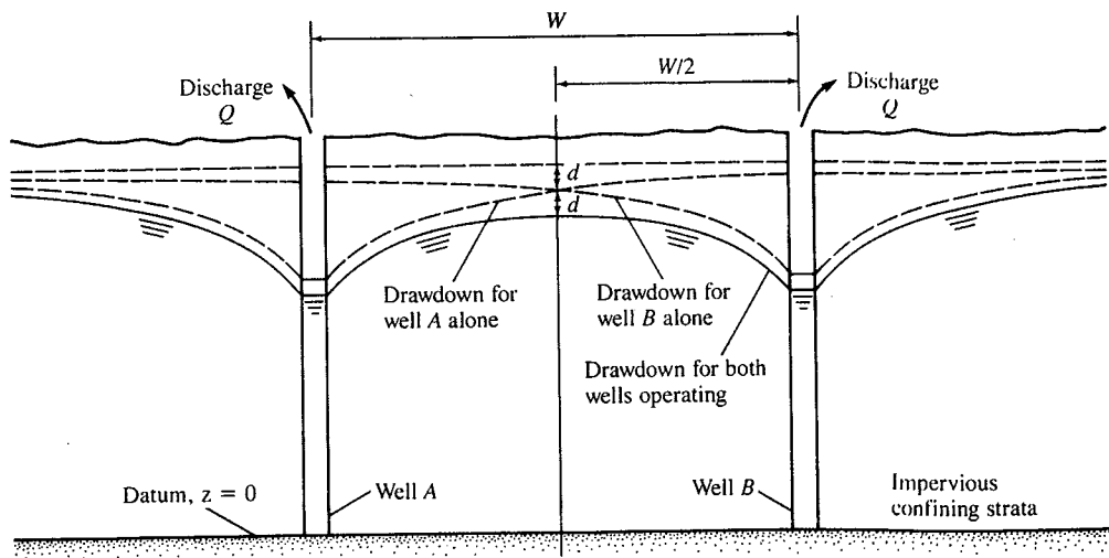
Figure 3-15 Determination of resultant drawdown for two pumped wells with mutual interference
