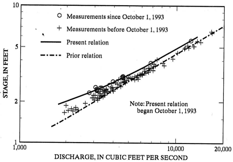
Figure 2.16 Sections of stage-discharge relations for the Colorado River at the Colorado-Utah State Line. (Wahl, Thomas, and Hirsch, 1995).
